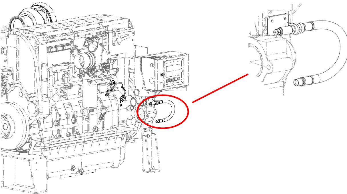
Figure 3-7 VSPLC pressure sensing connection
