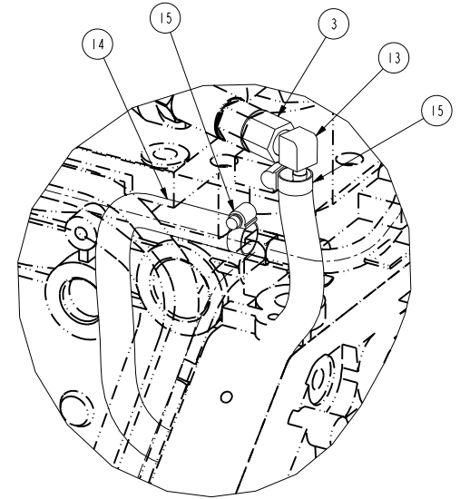
DETAIL A SCALE 0.625
