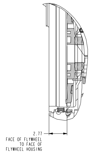
DETAIL B SCALE 0.250
